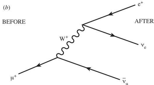
Figure 7. (a) The Feynman diagram for ordinary negative muon decay. (b) The diagram for positive muon decay.
